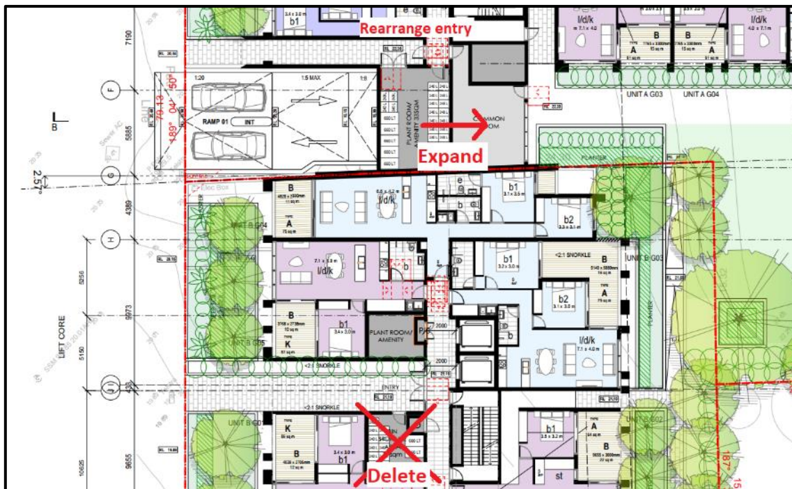
Figure 15. Ground Floor Plan diagram showing the proposed condition to consolidate the two bin rooms and improve accessibility.
