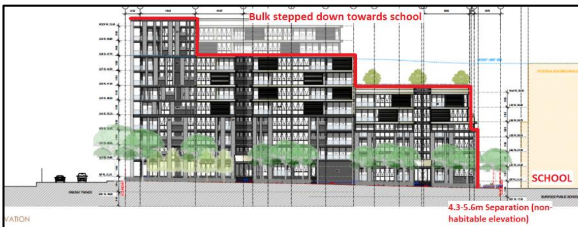
Figure 17. Marked amended northern elevation showing the stepped down bulk to minimise impacts on adjoining school (Source: Alexandar Design Group, 2018 / Marked: James Arnold, 2018)
